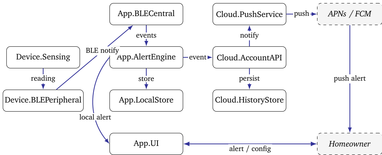
Figure 1: Device/app/cloud architecture carried forward from the ADS
